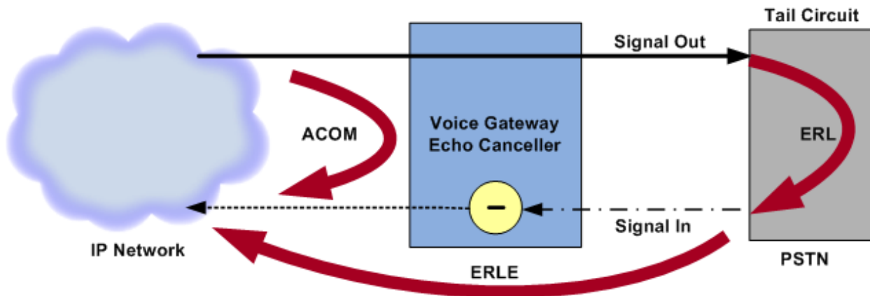
Figure 1. Echo Measurements & Echo Cancellation
